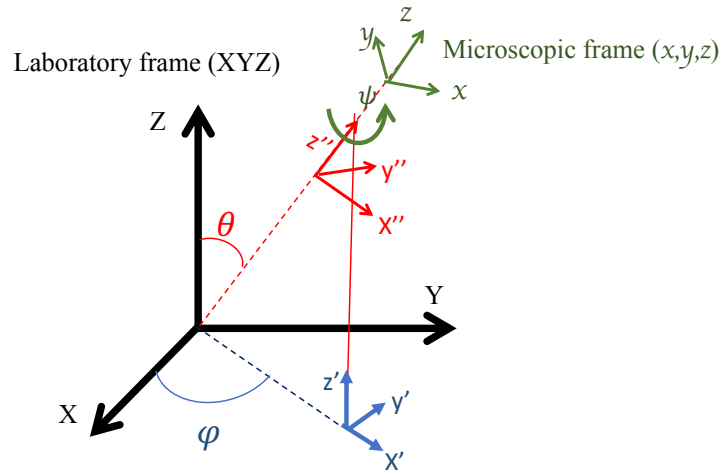
Figure 2: Definition of the angles \varphi, \theta, \psi which describe the orientation of the scattered object in the laboratory frame.
